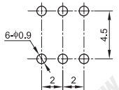
PCB LAYOUT (TOP VIEW)
