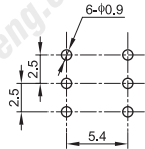
PCB LAYOUT (TOP VIEW)
