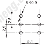
PCB LAYOUT (TOP VIEW)
