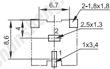
PCB LAYOUT (TOP VIEW)
