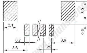
PCB LAYOUT (TOP VIEW)
