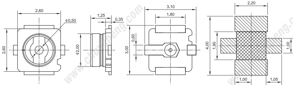
PCB LAYOUT (TOP VIEW)
