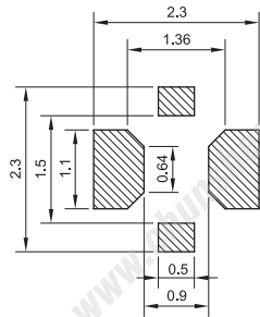
PCB LAYOUT (TOP VIEW)
