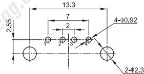
PCB LAYOUT (TOP VIEW)
