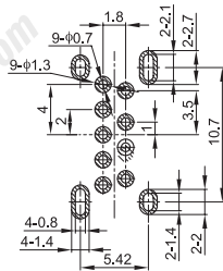
PCB LAYOUT (TOP VIEW)
